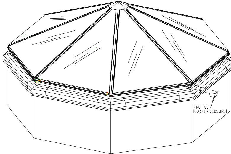
ASSEMBLED VIEW
