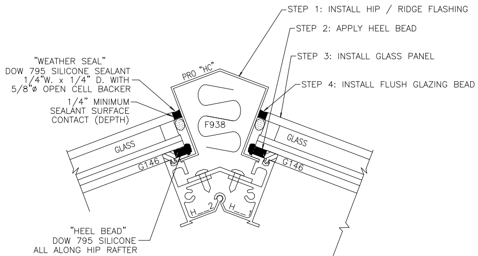
SECTION "A-A": SILICONE DETAILS @ HIP RAFTER
