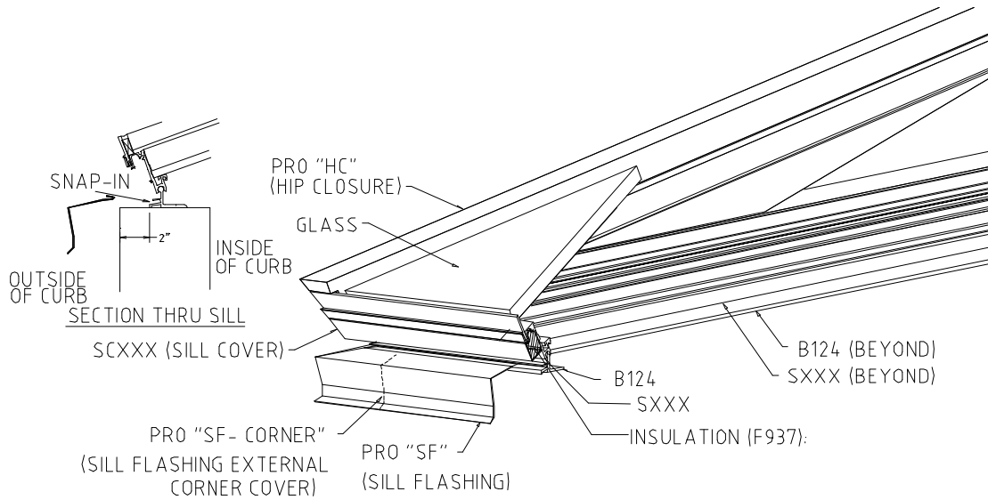
Diagram #14 – Sill Closure and Sill Flashing
