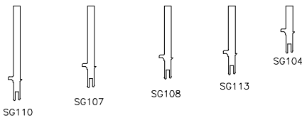
GLAZING SUPPORTS
