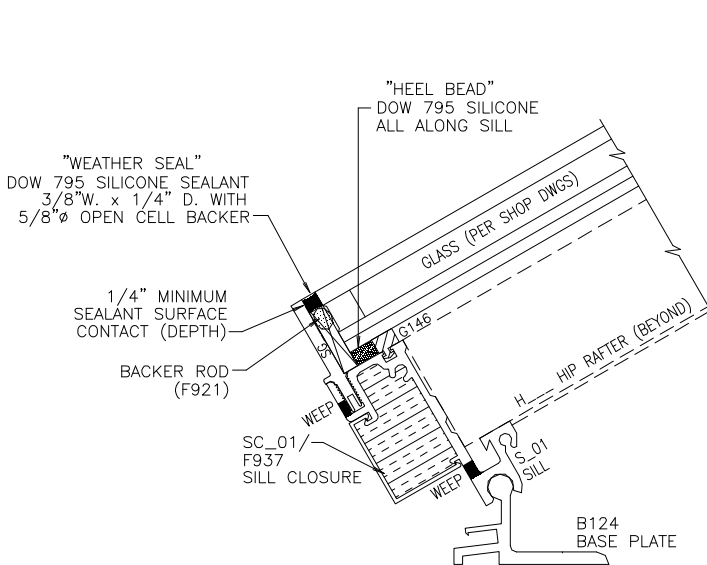
SILICONE DETAILS @ SILL
