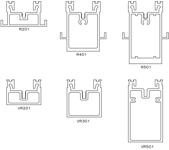
RAFTERS / MULLIONS
