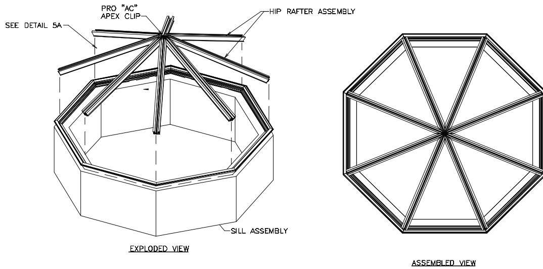
Diagram #5 – Hip rafter attachment @ apex
