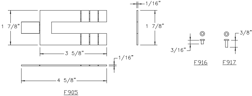
SHIM
