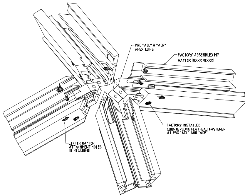
Diagram #5A – Hip rafter attachment @ apex
