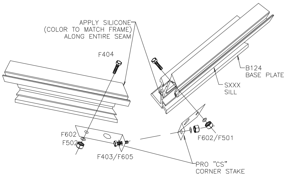
Diagram #3 – Attaching sill corner stakes
