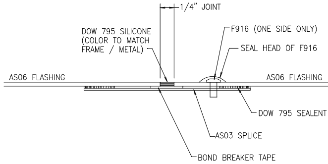
SPLICE DETAIL FOR 0.060" THICK MATERIAL
