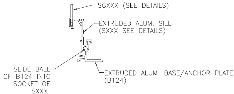
Diagram #2 – Attaching sill base plates
