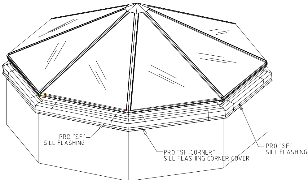
Diagram #14A – Sill Closure and Sill Flashing
