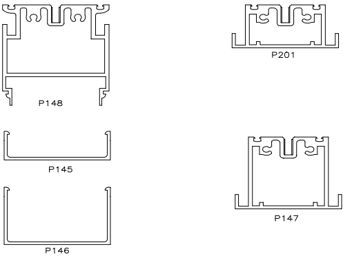
PURLINS
