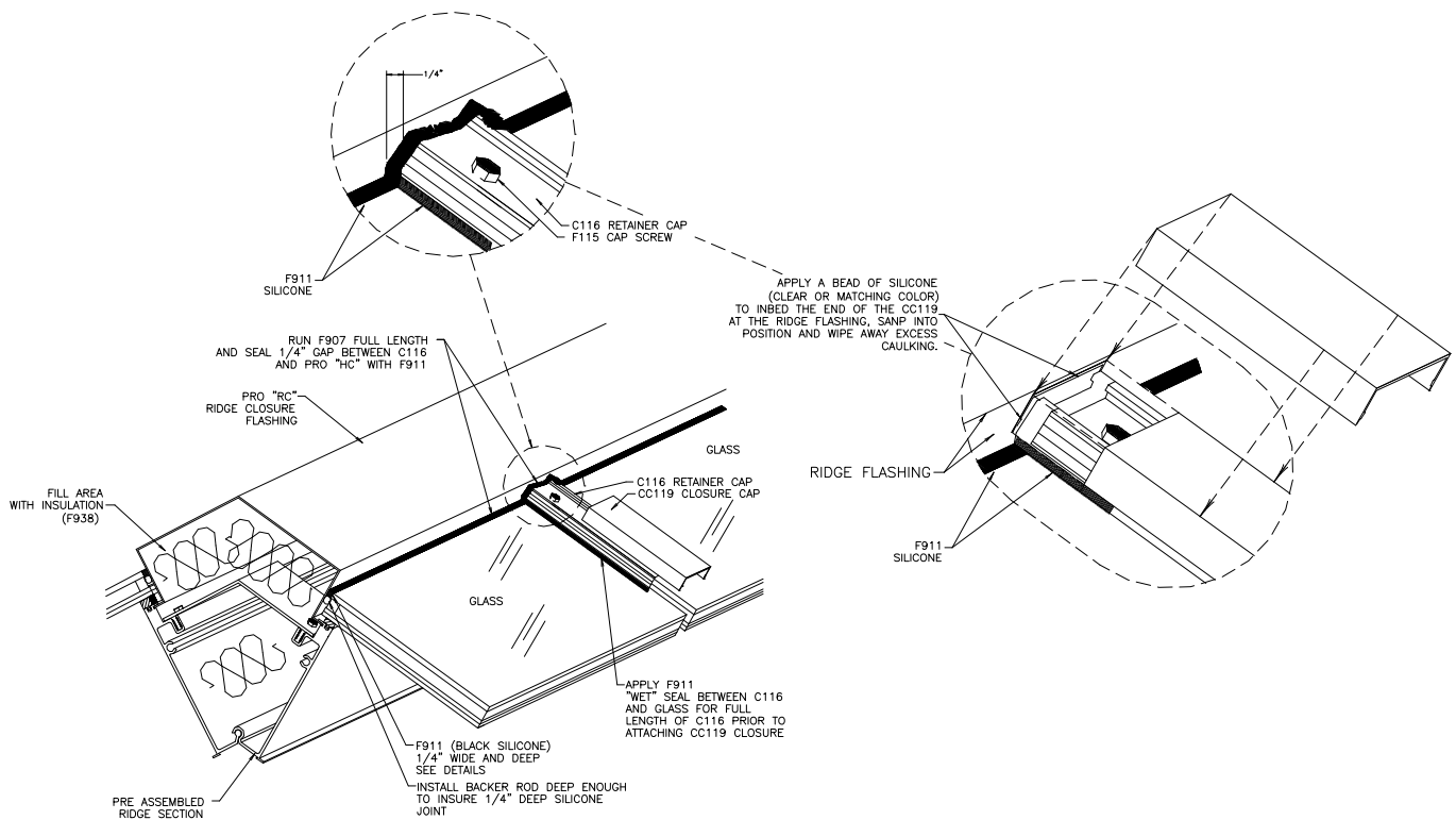
Diagram #11 – Cap installation @ hip rafter
