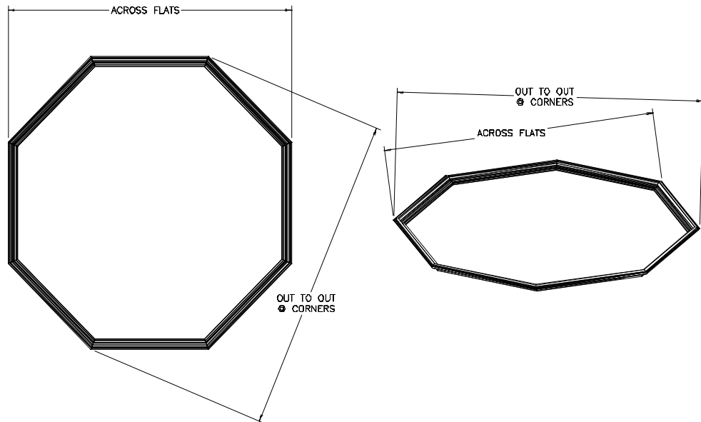
Diagram #3A – Checking sills for square
