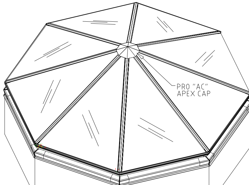
Diagram #13 – Apex Cap Assembly
