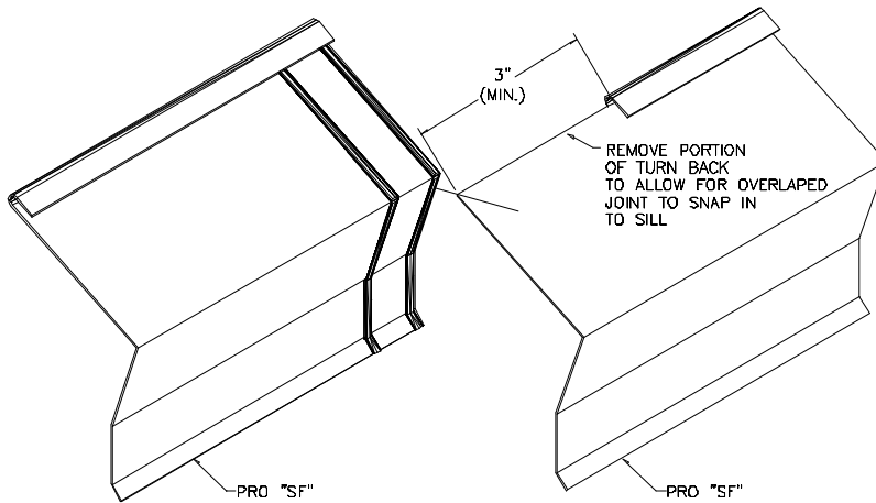
Diagram #15A – View of overlap flashing joint
