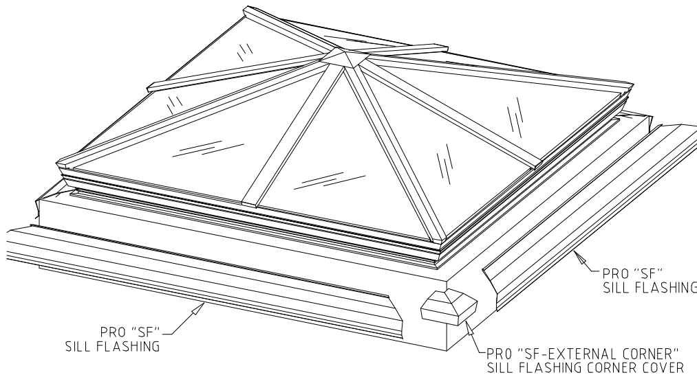
Diagram #14 – Sill Closure and Sill Flashing
