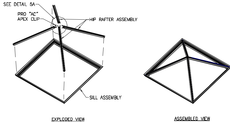
Diagram #5 – Hip rafter attachment @ apex
