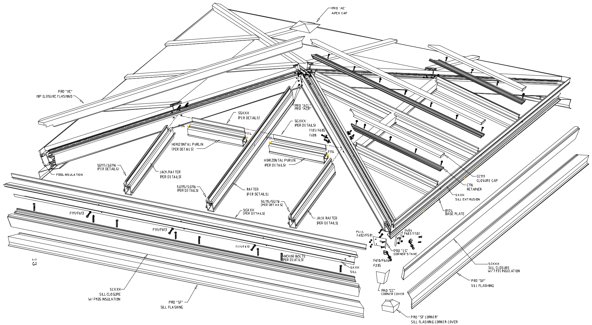
Exploded View of Pyramid
