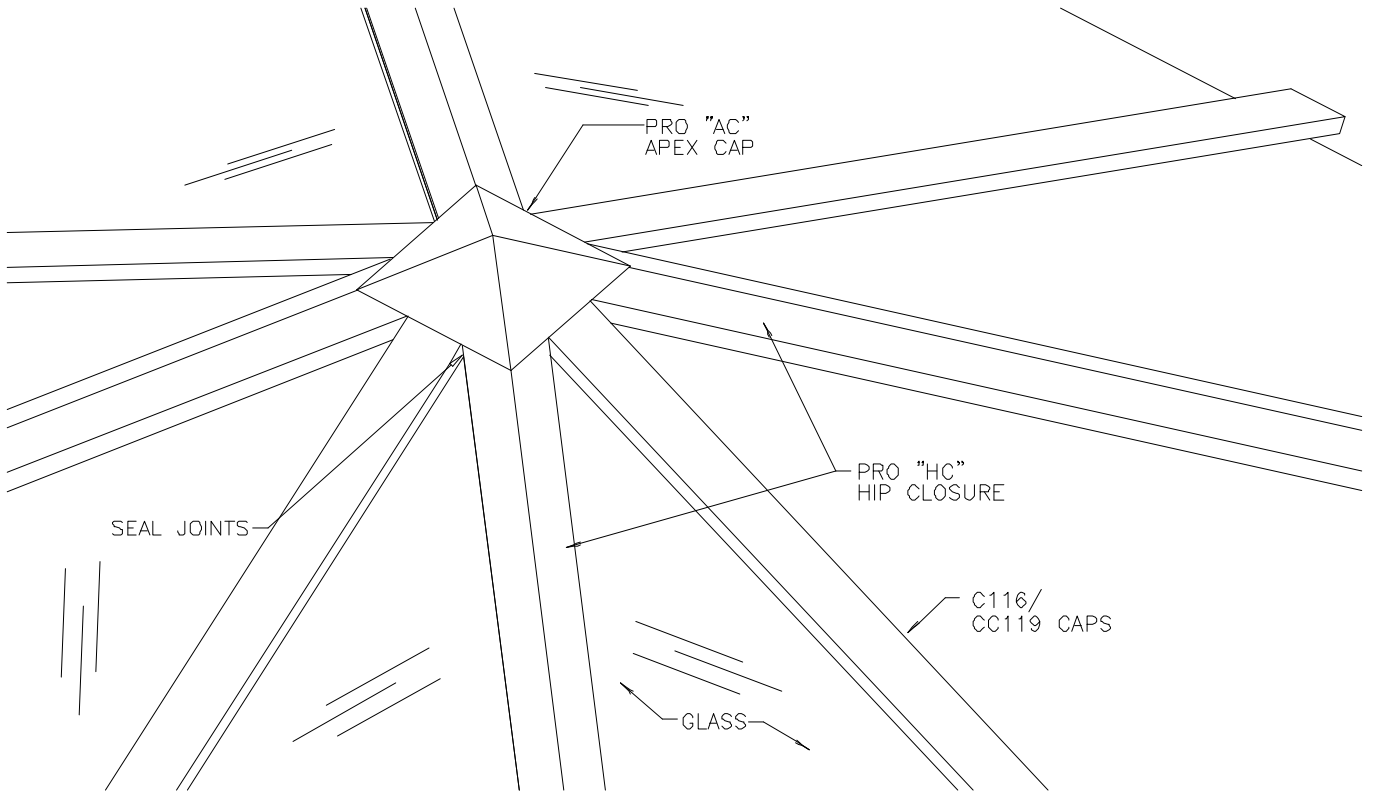
Diagram #13 – Apex Cap Assembly
